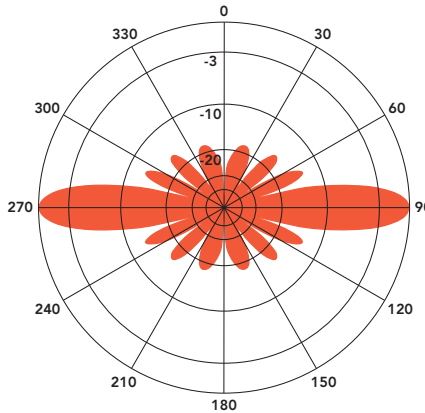
ANT440F6 - 450 MHz Vertical Plane Gain = 6.22 dBd
