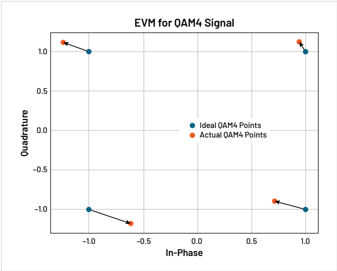
Figure 6 – QAM4 Error Vectors.
