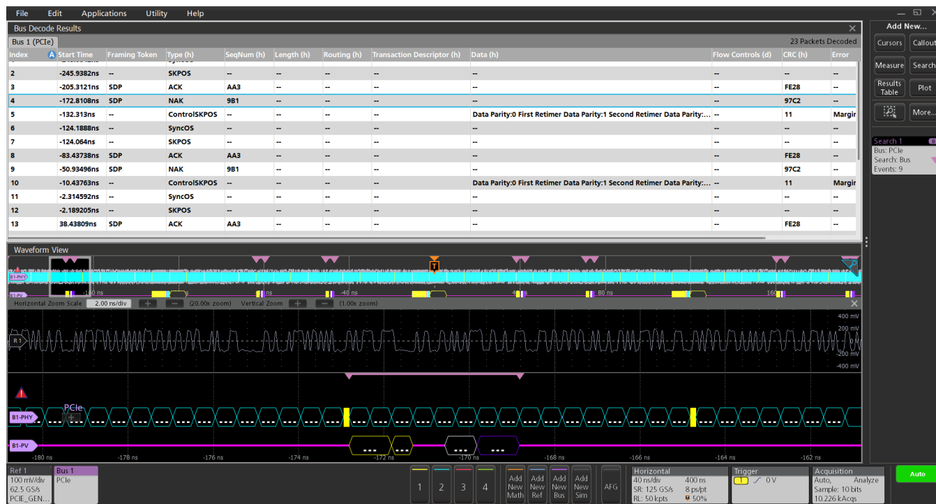
Triggering on a PCIe Gen4 high-speed serial bus with decoded packet display.
