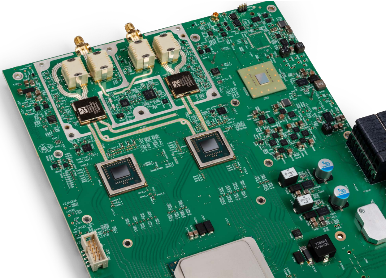
New high-performance signal path utilizing custom ASIC technology.
