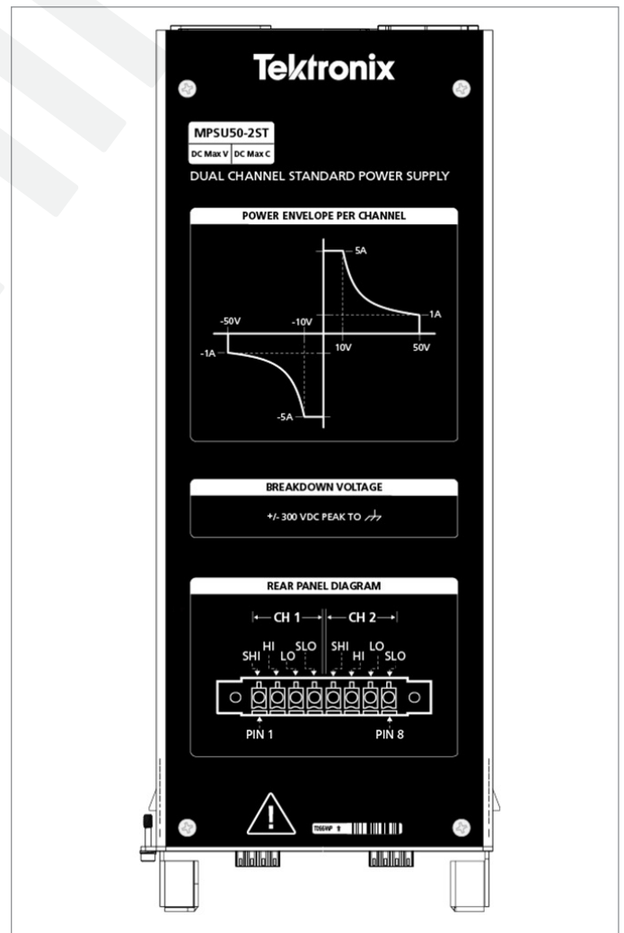
Figure 2: MPSU50-2ST Module
