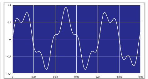
Interharmonics Waveform
